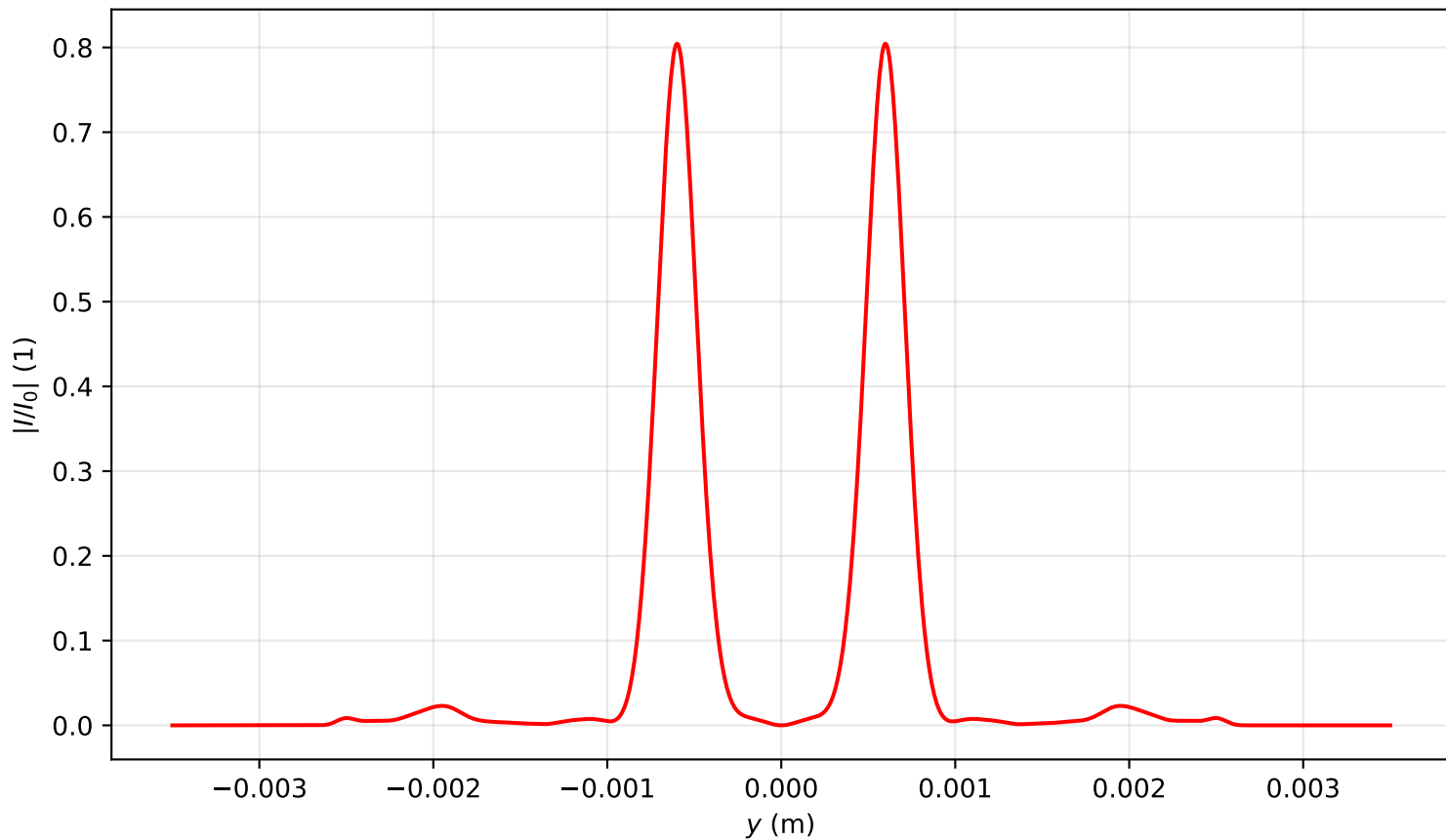
Intensity profile I(x=0, y, z=1.751)/I_0 , P_{in}=8.0P_{cr} , artificial time
